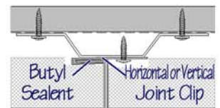
Met-Flush II Flush vertical & horizontal wall panel system (limited applications)
