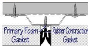
Metposite STD-DRI-RS Gasketed (rain screen) wall and soffit panel system
