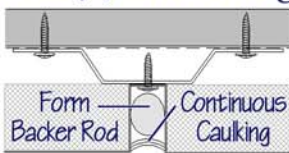
Metposite STD Backer rod and caulk wall and soffit panel system
