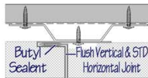
Met-Flush Flush vertical joint wall panel system
